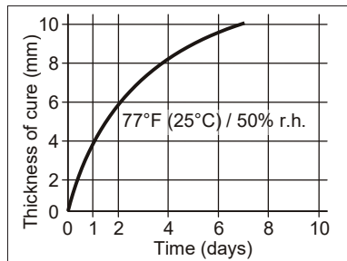
Diagram 1: Curing speed Sikasil®-N Plus US
