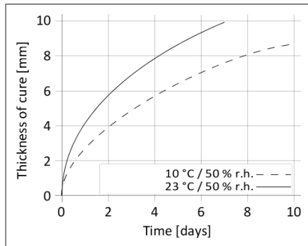
Diagram 1: Curing speed Sikasil® GP-101
