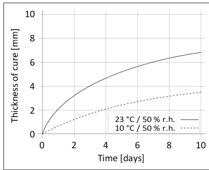
Diagram 1: Curing speed of Sikaflex®-511
