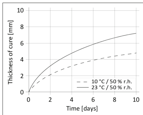
Diagram 1: Curing speed of Sikaflex®-510 AM50
