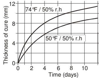
Diagram 1: Curing speed Sikaflex®-265
