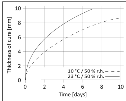
Diagram 1: Curing speed Sikaflex®-227 US
