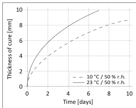
Diagram 1: Curing speed Sikaflex®-219 LM
