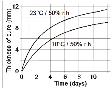
Diagram 1: Curing speed Sikaflex®-124 Mirror Grip
