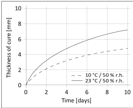
Diagram 1: Curing speed of Sikaflex®-510 AM50
