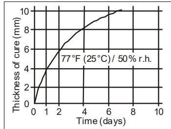
Diagram 1: Curing speed Sikasil® SG-10
